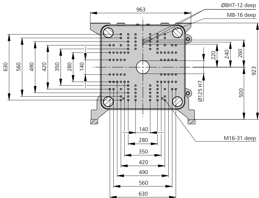
Fixed mould mounting platen | A
